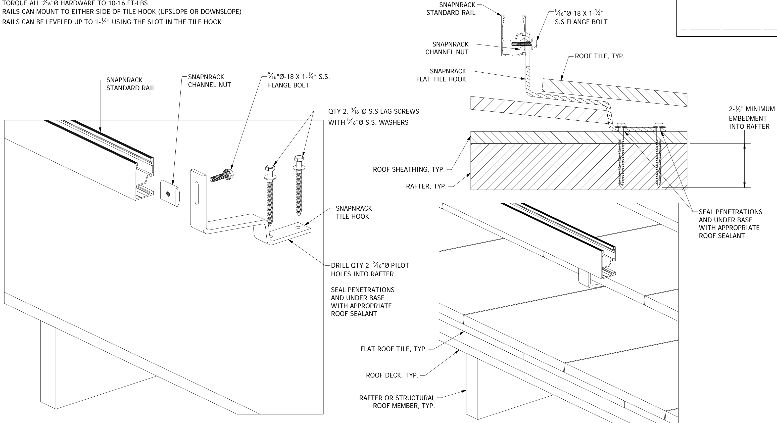
COMPLETED INSTALLATION
