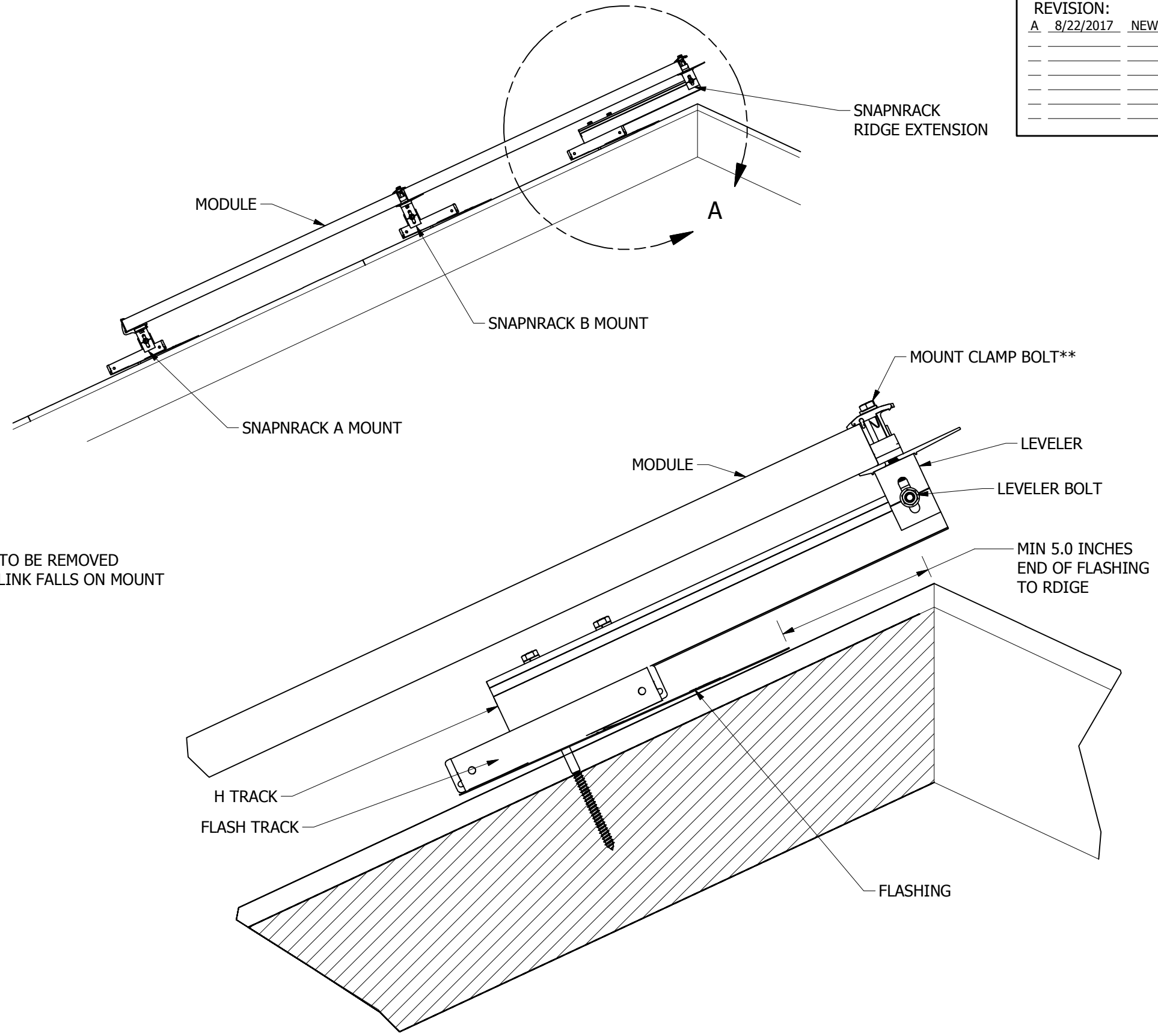
DETAIL A
