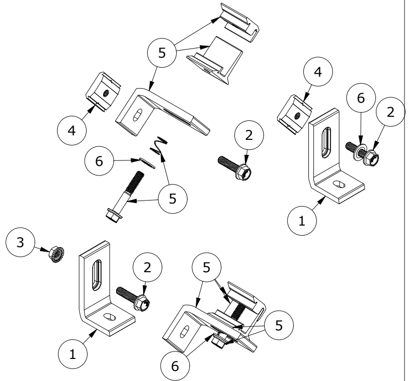
EXPLODED SCALE 1:4
