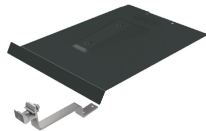
Tile Roof Hook F & Flat Tile Hook Replacement Flashing 242-01247 & 232-60055
