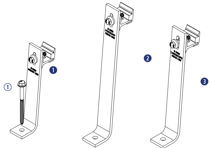
EXPLODED VIEWS
