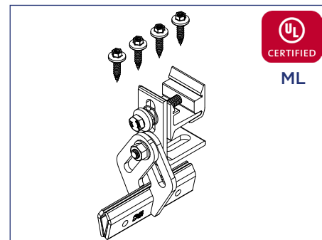
S-5! ProteaBracket with Ultra Rail hardware
