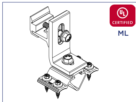
S-5! CorruBracket 100T with Ultra Rail hardware
