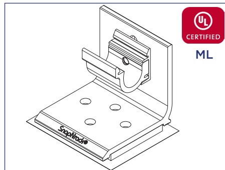
UltraFoot, Deck Roof Attachment Roof attachment kit for composition shingle roofs including chemically flashed L foot and hardware
