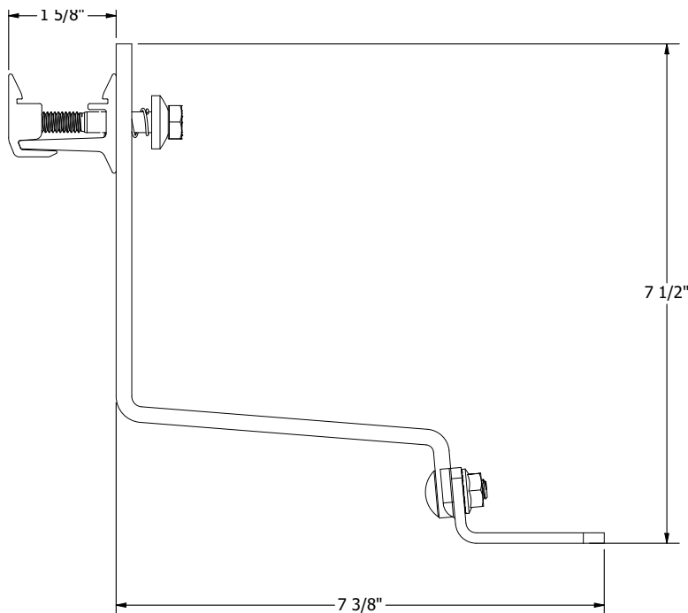
Dimensioned Ultra Rail Adjustable Tile Hook Assembly
