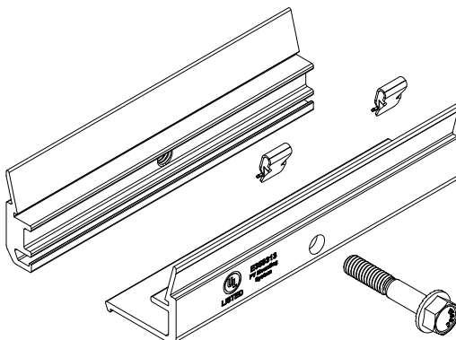
UR-40 & UR-45 Rail Splice
