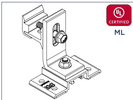
S-5! SolarFoot with Ultra Rail hardware
