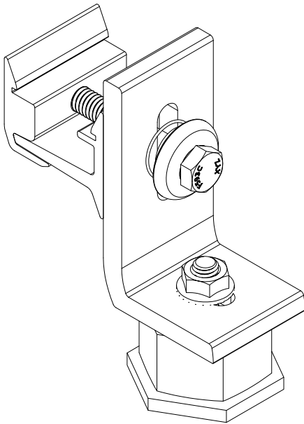
Ultra Rail Mounting Hardware Installed on Different Roof Attachments
