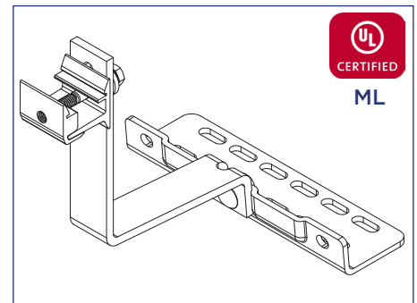
Tile Roof Attachment Roof attachment kit for W, S, and Flat tile roofs including adjustable height tile hook, base, and hardware
