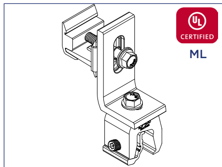
S-5-N-mini with Ultra Rail hardware
