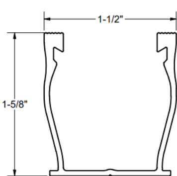
UR-40 Rail Profile
