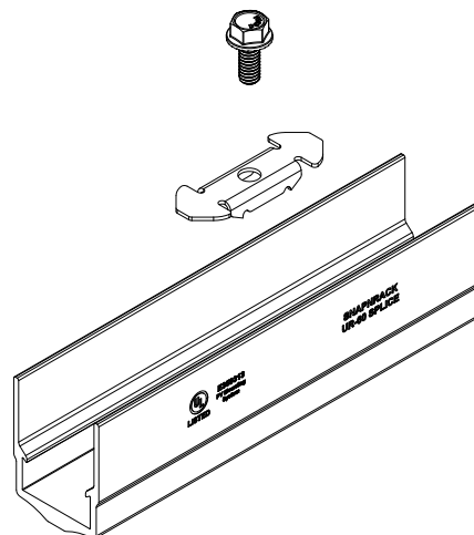
UR-60 Rail Splice
