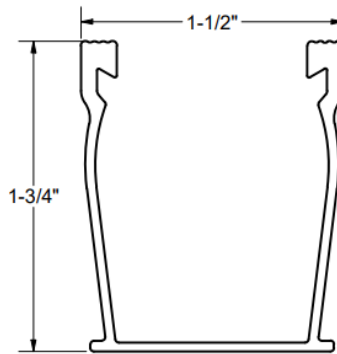
UR-45 Rail Profile
