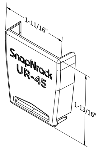
Dimensioned UR-45 Rail End Cap
