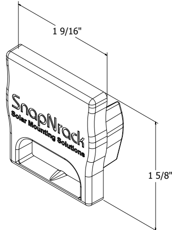
Dimensioned UR-40 Rail End Cap
