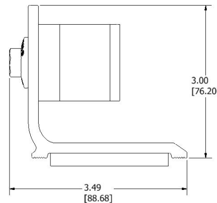
Dimensioned UltraFoot™ Deck
