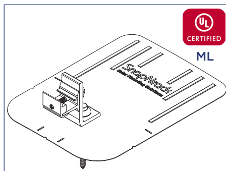
Umbrella L Foot Roof Attachment Roof attachment kit for composition shingle roofs including L foot, umbrella lag screw, flashing, and hardware
