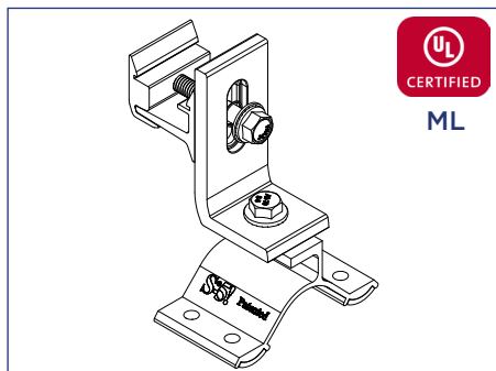
S-5! CorruBracket with Ultra Rail hardware
