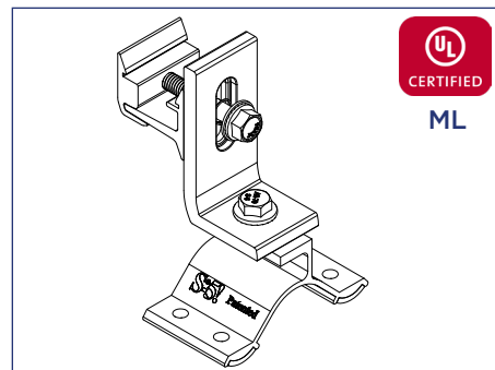
S-5! VersaBracket with Ultra Rail hardware
