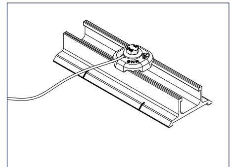
3) Each continuous array is connected to Equipment Grounding Conductor through OmniLug installed on one Flash Track, SpeedSeal™ Track, or SpeedSeal™ DeckTrack per array
