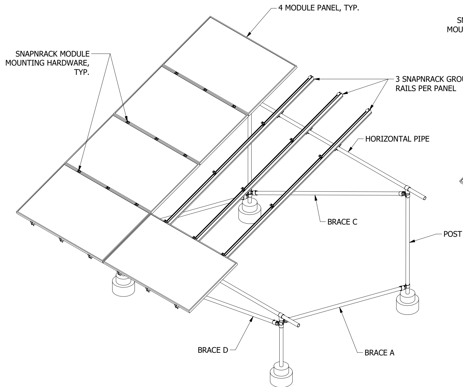
4 MODULE PANEL CONFIGURATION
