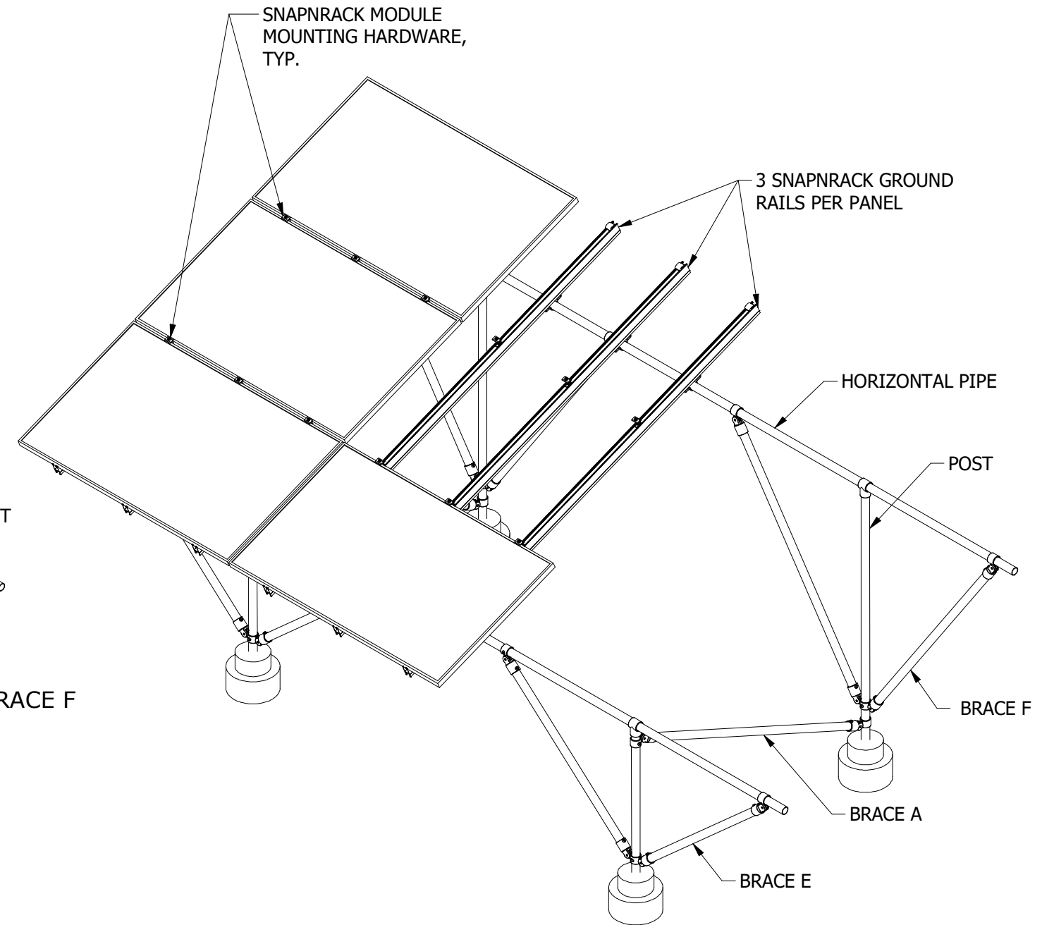
3 MODULE PANEL CONFIGURATION
