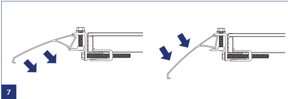
7 (1) Pull Universal Skirt up into top of Skirt Mount, (2) then push the Skirt down to snap it into the mount.
