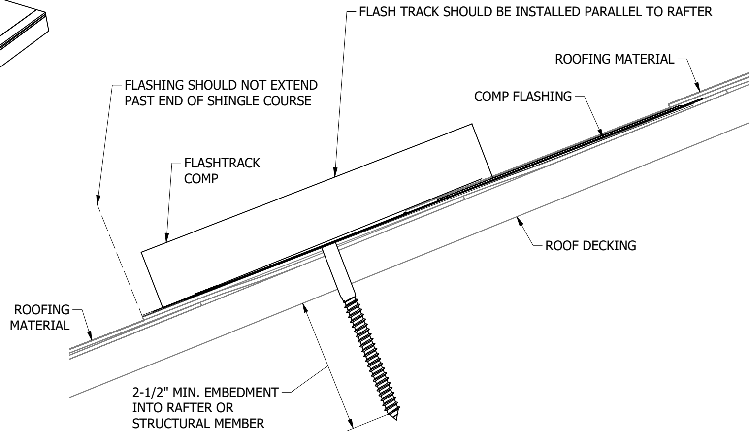
COMPLETED INSTALLATION
